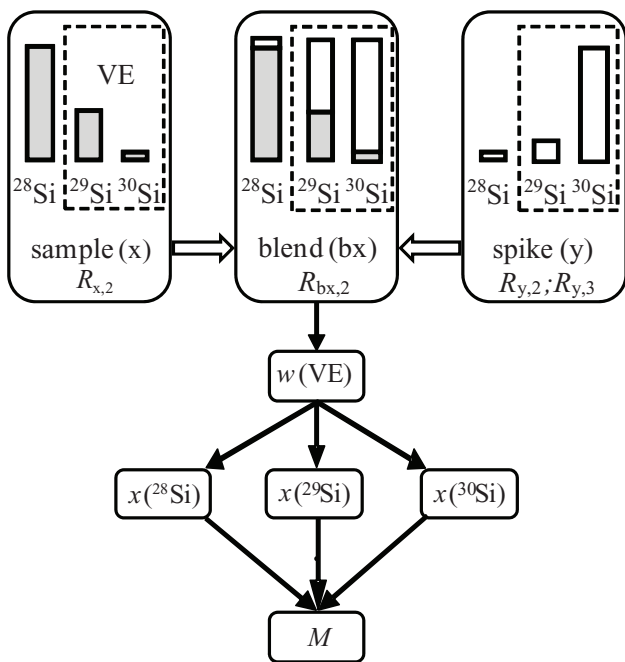
Figure 9. VE-IDMS principle: the VE consists of the 29 Si and 30 Si isotopes (dashed frame). The isotope ratios R = x(^{30}\text{Si})/x(^{29}\text{Si}) are measured in the sample, blend, and spike, yielding the mass fraction w(\text{VE}) = w(^{29}\text{Si}) + w(^{30}\text{Si}) , that in turn yields all x(^i\text{Si}) and M .
