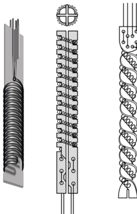
Figure 3. Schematic designs of sensitive elements of SPRTs: HTSPRT with a simple bifilar platinum coil supported on a notched high-purity silica plate, R(0.01\text{ °C}) \sim 0.25\text{ Ω} (left); LSPRT with the platinum coil laid in notches in a silica cross, R(0.01\text{ °C}) \sim 25\text{ Ω} (centre and top-view); LSPRT with the platinum coil laid in the helical turns of a twisted silica plate, R(0.01\text{ °C}) \sim 25\text{ Ω} (right). In all cases two platinum wires are welded to the coils at each end to create four-lead connections (“Y” joints). (Illustration published on courtesy from FLUKE®)
