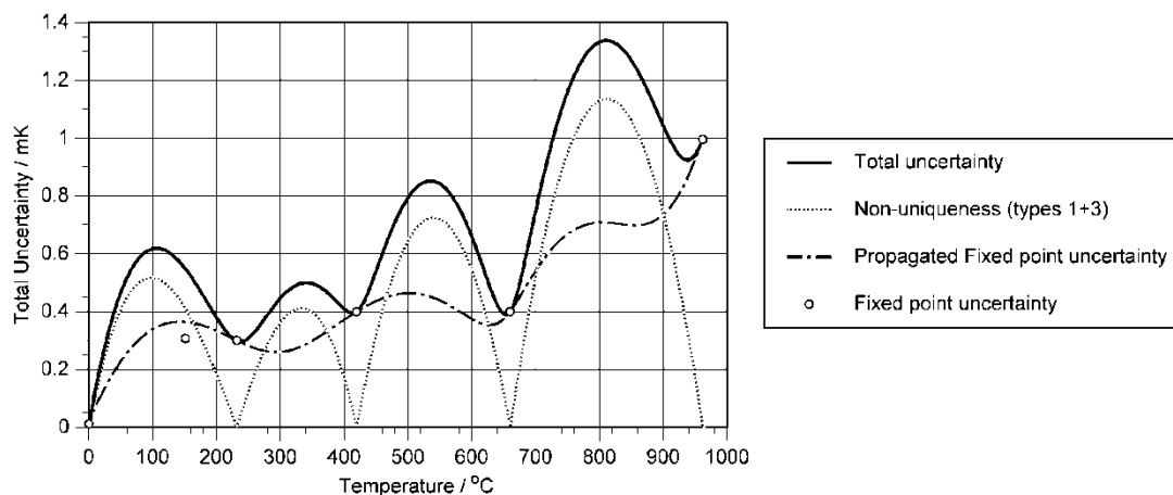
Figure 13: Example of the total calibration uncertainty for a SPRT over the water-silver sub-range, showing the contribution of uncertainty due to fixed points and the two forms of non-uniqueness. The values shown are standard uncertainties and are indicative of a high-quality ITS-90 realisation.
