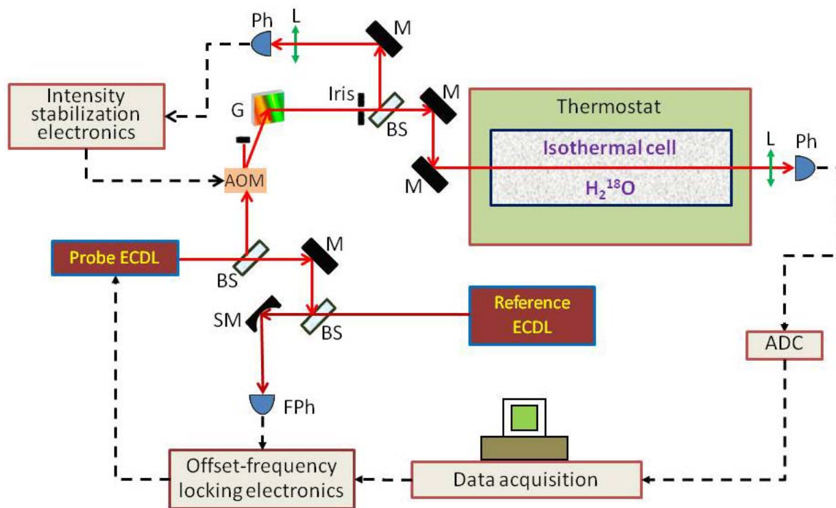
Figure 1. Sketch of the laser absorption spectrometer developed at the wavelength of 1.39\ \mu\text{m} . M stands for mirror, L for lens, SM for spherical mirror, BS for beam-splitter, Ph for photodiode, FPh for fast photodetector, G for diffraction grating, AOM for acousto-optic modulator, ADC for analog-to-digital converter.
