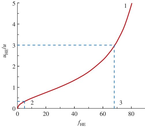
Fig. 3: Ratio of the uncertainty due to residual risk of human errors u_{\text{HE}} to the measurement uncertainty u in dependence on % of the quality loss f_{\text{HE}} (line 1). The cases u_{\text{HE}} = 1/3u and u_{\text{HE}} = 3u are indicated by dotted lines 2 and 3, respectively. ©Bureau International des Poids et Mesures. Reproduced from Ref. [42] by permission of IOP Publishing. All rights reserved.
