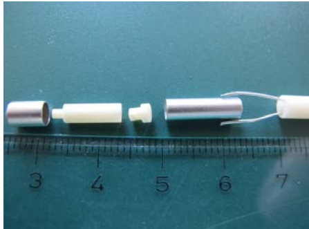
Figure 10: Miniature fixed point welded between the thermoelements
