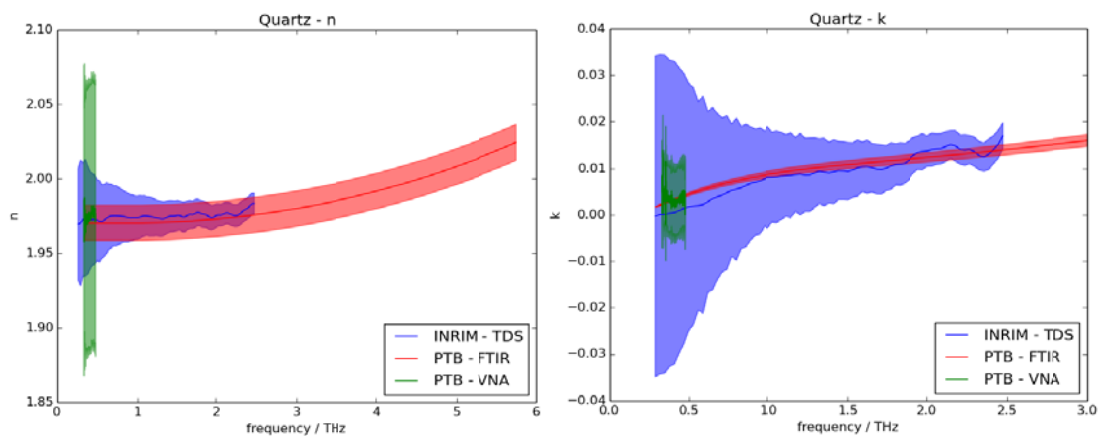
Figure 4. Comparison of measurement results for the quartz travelling standard.
