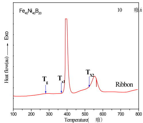
Figure 2. DSC curves of \text{Fe}_{40}\text{Ni}_{40}\text{B}_{20} amorphous ribbon
