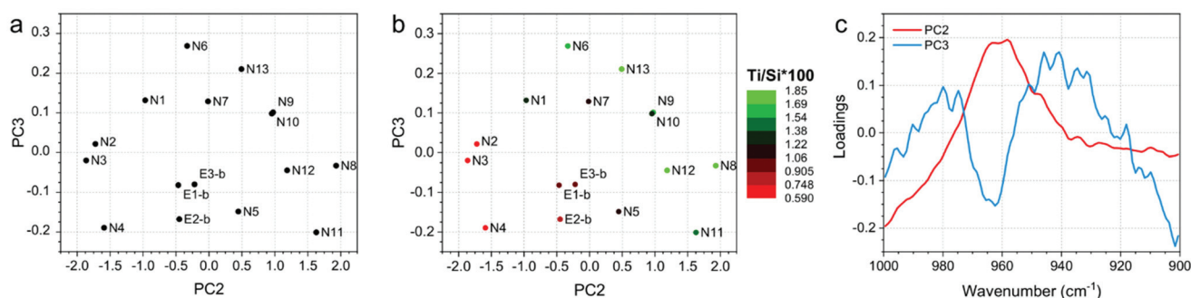
Fig. 4 (a) PC2 and PC3 scores plot, (b) PC2 and PC3 scores plot, in which the sample spots were scaled according to the Ti/Si × 100 and (c) loadings plot of the PCA model developed on ATR-IR data.
