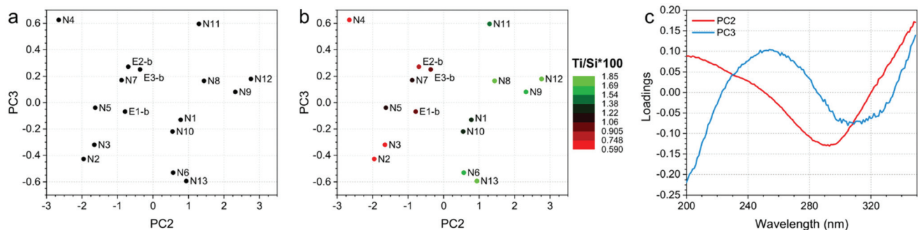
Fig. 5 (a) PC2 and PC3 scores plot, (b) PC2 and PC3 scores plot, in which the sample spots were scaled according to the Ti/Si × 100 and (c) loadings plots of the PCA model developed on DR-UV data.
