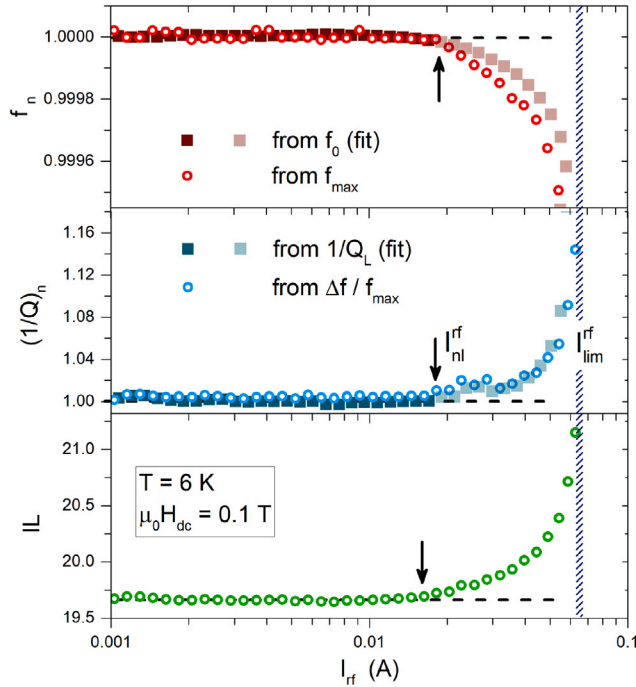
Fig. 3. Resonance frequency, normalized by its low-power value (a), inverse of the loaded quality factor, normalized by its low-power value (b), and insertion loss (c) as a function of the rf current circulating in the CPWR at the resonance, calculated by Eq. (2). Data were extracted from Lorentzian fits of the resonance curves ( f_0 , Q_L ) and directly from the experimental S_{21}(T) resonance curves (frequency at the maximum, f_{max} , curve width at -3 dB, \Delta f ), insertion loss IL = -20\text{Log}(|S_{21}|^{max}) . The limiting rf current I_{lim}^{rf} is the maximum current flowing in the CPWR.
