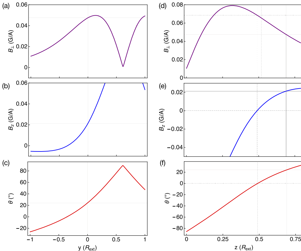
FIG. 6. Simulated spatial profile of the B -field generated by the RF coil for a current of 1 \text{ A}_{\text{pp}} flowing through the coil. (a) and (b) Transverse and axial RF-field amplitudes, B_{\perp} and B_z , along the y -axis at (x, z) = (0, |d|) . (c) B -field vector angle with respect to the x - y plane along the y -axis. (d) and (e) Transverse and axial RF-field amplitudes, B_{\perp} and B_z , along the z -axis at (x, y) = (0, 0) . (f) B -field vector angle with respect to the x - y plane along the z -axis. The position of the atomic sample is (x, y, z) \simeq (0, 0, |d|) with |d| \simeq 0.7R_{\text{ext}} , as denoted by solid vertical grid lines. Dashed vertical grid lines denote the optimal coil distance from the atomic sample to obtain a B -field perpendicular to the z -axis at (x, y) = (0, 0) .
