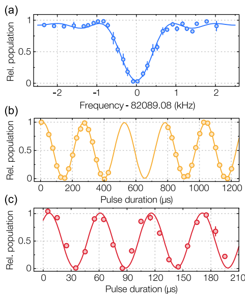
FIG. 5. System performance measured with an ideal Fermi gas of ^6\text{Li} atoms at B_0 \simeq 770 G. On the vertical axis, the relative population denotes the number of atoms in state |2\rangle normalized to the total atom number. (a) Spectroscopy of the |2\rangle \leftrightarrow |3\rangle transition. The solid line is a fit of the data with the expected sinc-function line shape, yielding a resonance frequency \nu_0 = 82.089\,08(1) MHz and a Rabi frequency \Omega_R/2\pi = 410(16) Hz. (b) and (c) Rabi oscillations at the resonance between states |2\rangle and |3\rangle for RF generator powers of about 3.5 W (yellow) and 80 W (red). Solid lines are sinusoidal fits to the data, yielding Rabi frequencies \Omega_R/2\pi = 3.909(4) kHz and \Omega_R/2\pi = 18.25(23) kHz, respectively.
