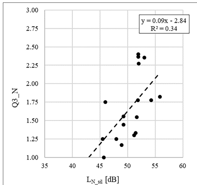
FIGURE 2 | Linear regression graph showing the dependency of the average values across classes of the answers to the question Q3_N (i.e., "How much sounds of radios or recorders coming from other classrooms or from the corridor disturb you?") on the noise level measured with children in silence, L_{N\_sil} .
