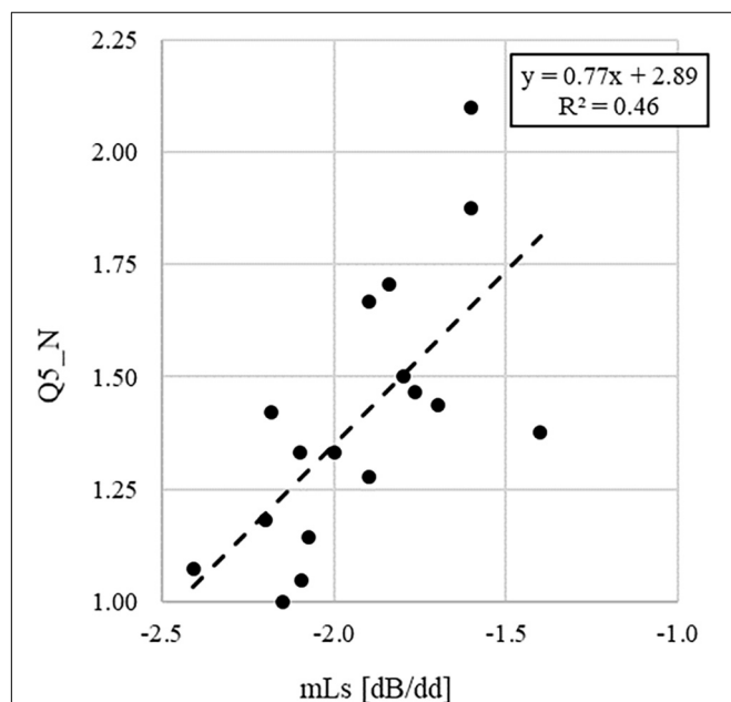
FIGURE 3 | Linear regression graph showing the dependency of the average values across classes of the answers to the question Q5_N (i.e., "The noise present when you perform a task in silence seems you.") on the slope of the voice signal, mLs .
