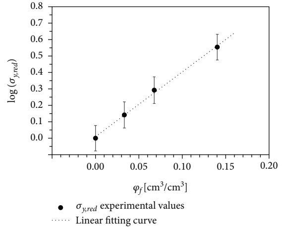
FIGURE 4: Relative tensile stress at yield, \sigma_{y,rel} , calculated according to the Pukanszky's model, as a function of the ZTC volumetric fraction.
