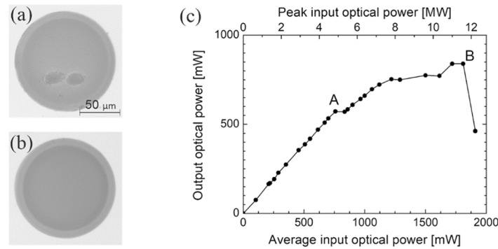
Fig. 4. Optical microscope photographs of the input fiber connector with 105/125 μm MM fiber: (a) connector damage when using ~20 μm spot size of the test beam, (b) the connector after tests with ~40 μm spot size of the test beam. (c) Optical power transmitted through the MM optical fiber spliced to MM CPG fiber for the pulsed laser system at 532 nm. The beginning of damage of the fiber is marked as A, while the detrimental break is marked as B. A line connecting the points is plotted just as an eye-guide.
