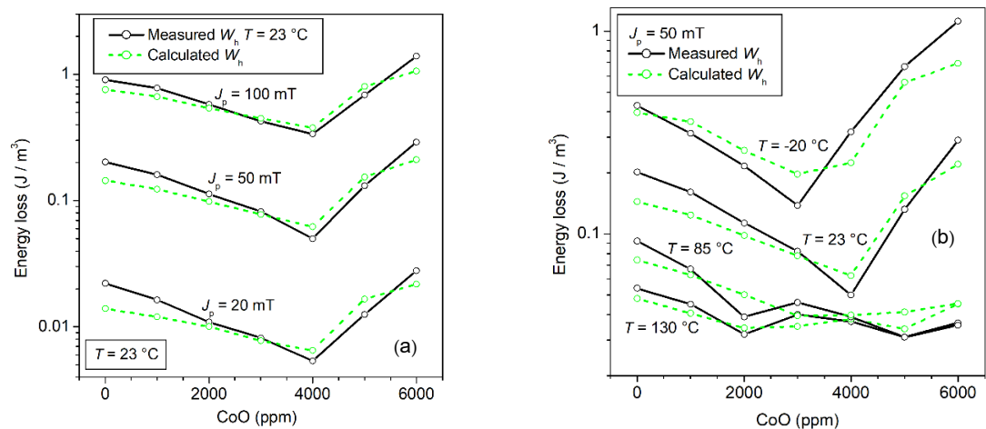
Figure 13. (a) The hysteresis energy loss W_h measured at T = 23^\circ\text{C} versus CoO content at different J_p values is compared with the prediction made through Equation (7). We make use in this equation of the experimental quantities \langle K_{\text{eff}} \rangle (Figure 12b), J_s , \mu_{\text{rot,DC}} , \mu_{\text{dW,DC}} , and \langle s \rangle , and a parameter a(J_p) \sim \propto J_p^{1.1} , independent of the CoO content. (b) The same predicting equation leads to the calculated W_h versus CoO at defined J_p value and different temperatures, broadly reflecting the evolution of \langle K_{\text{eff}} \rangle in Figure 12b at such temperatures. (Adapted from Ref. [42]).
