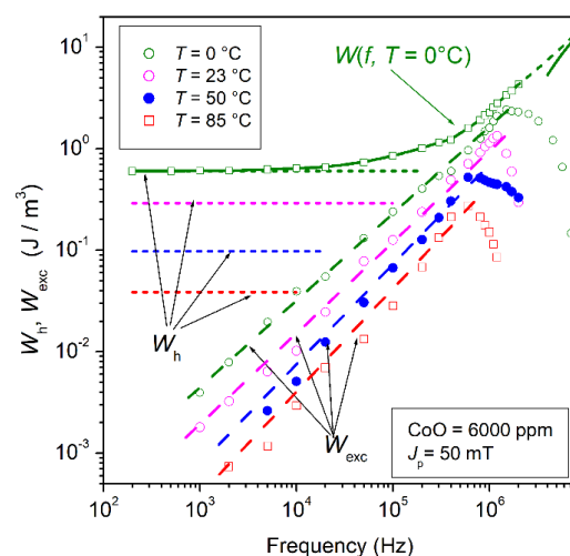
Figure 16. Hysteresis W_h and excess W_{\text{exc,sd}}(f) loss components versus temperature ( J_p = 50 \text{ mT} , T = 0, 23, 50, 85^\circ\text{C} ) in a 6000 ppm CoO-doped Mn-Zn ferrite. The decrease in the effective anisotropy with increasing T justifies the associated decrease in the dw-related loss contributions. The correlation between the W_h and W_{\text{exc,sd}}(f) dependences on T confirms that both quasi-static and dynamic dw displacements respond the same way to strength and distribution of the pinning fields. (Partly adapted from Ref. [42]).
