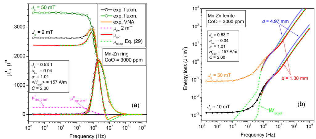
Figure 6. (a) The rotational permeability components \mu'_{rot}(f) and \mu''_{rot}(f) are singled out in a CoO-doped Mn-Zn ferrite ring sample, following the scheme provided by Equations (19)–(23). The symbols and the solid lines are the results of fluxmetric (exp. fluxm.) and transmission line (exp. VNA) measurements. They are theoretically calculated using Equations (29a) and (29b) (dashed lines) with lognormal distribution function for the effective anisotropy field strength H_{k,eff} (average value \langle H_{k,eff} \rangle ). The parameters of the distribution, given in the inset, are the width \sigma and the constant C (Equations (27) and (31)). \alpha_{LL} is the Landau–Lifshitz damping constant. (b) The corresponding rotational loss by spin damping W_{rot,sd}(f) is obtained from the calculated rotational permeabilities by means of Equation (13). The additional contribution by eddy currents is observed beyond a few MHz in the thicker sample ( d = 4.97 mm).
