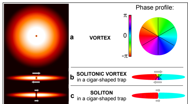
FIG. 2. (color online) Theoretical solutions of in-situ density and phase profiles for: (a) a vortex aligned along the axis of an axially symmetric potential, a solitonic vortex (b) and a soliton (c) oriented perpendicularly to the axis of an elongated axially symmetric trap. Arrows indicate the atomic flow.
