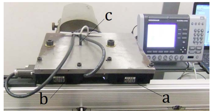
Figure 5. Bislider close-up. (a)(b) Heads; (c) Pt100. Spacing b = 137 mm.
