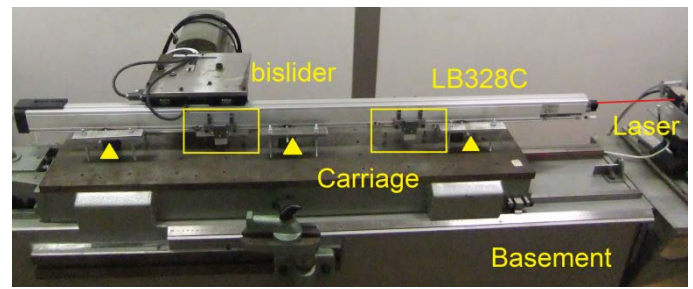
Figure 4. Measurement setup. Triangles: supports; rectangular frames: straining devices.
