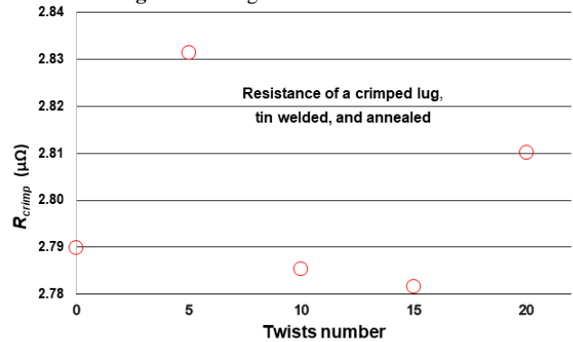
Fig.15. R_{crimp} behaviour of a lug crimped to a cable undergoing rotations on and around the lug plane.
