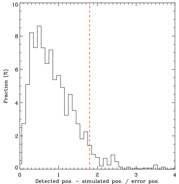
Fig. 1. Distribution of the difference between the detected X-ray positions and the input positions in units of the X-ray positional error.
