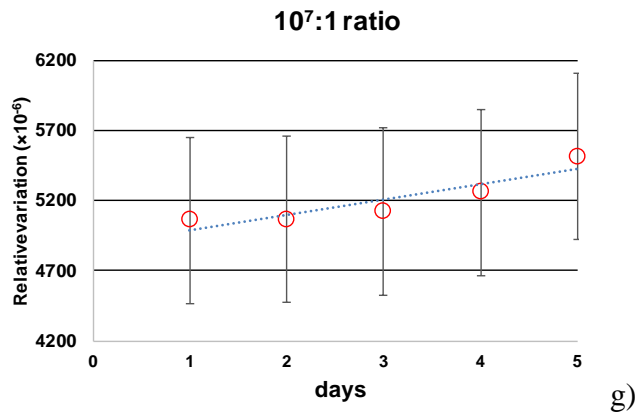
Fig. 8. Divider short-term (5 days) drift in ratio a) 10:1, b) 100:1, c) 10 3 :1, d) 10 4 :1, e) 10 5 :1, f) 10 6 :1 g) 10 7 :1. The uncertainty bars corresponds to the expanded calibration uncertainties.
