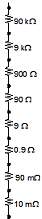
Fig. 1) Divider scheme
