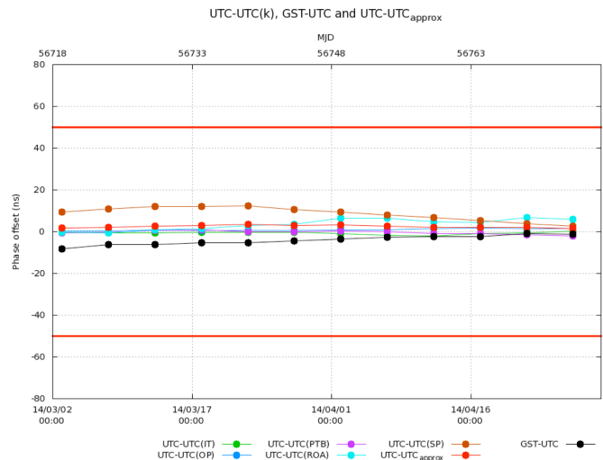
Fig. 7. Performance of UTC-UTC(k) from Circular T for the five laboratories contributing to the TVF. The evolution of UTC-UTCapprox and GST-UTC is also shown.
