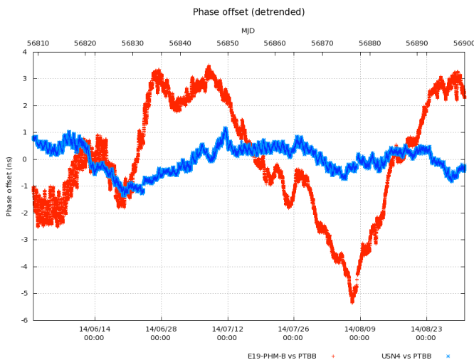
Fig. 8. E19 PHM-B satellite clock offset evolution over one quarter (91 days), versus PTBB. The USN4 clock evolution is also shown.
