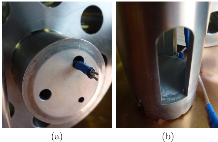
Figure 4: R1233zd(E) polymers deposited on the pressure vessel top stopper (a) and on the reflector of the measurement cell (b).
