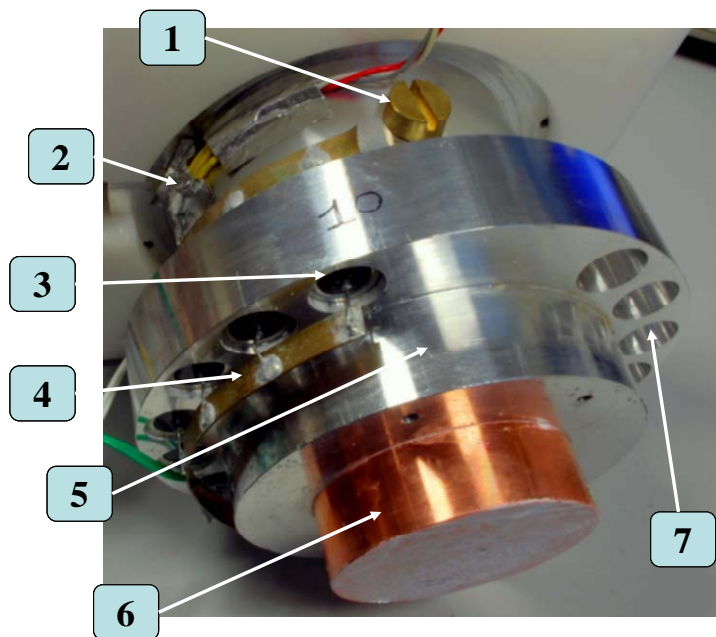
Fig.2. The structure of the 1 \Omega and 10 \text{ k}\Omega : 1) cap to insert mineral oil; 2) electronic thermometer; 3) ten 100 \text{ k}\Omega resistors inserted in the holes of the aluminium structure; 4) manganin strip for parallel connection; 5) cylinder containing the ten 10 \Omega resistors connected in parallel; 6) copper collector between the cylinder and the TEC where are inserted a thermometer and a PT100 platinum sensor for temperature control ( 10 \text{ k}\Omega NTC); 7) available empty holes for eventual compensation resistors.
