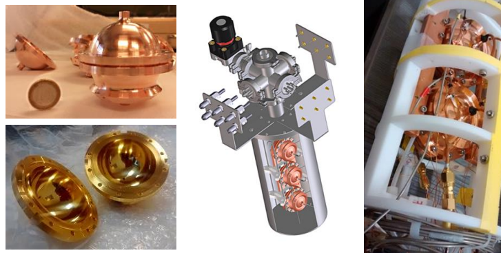
Figure 4: second generation of microwave hygrometers and their assembly
