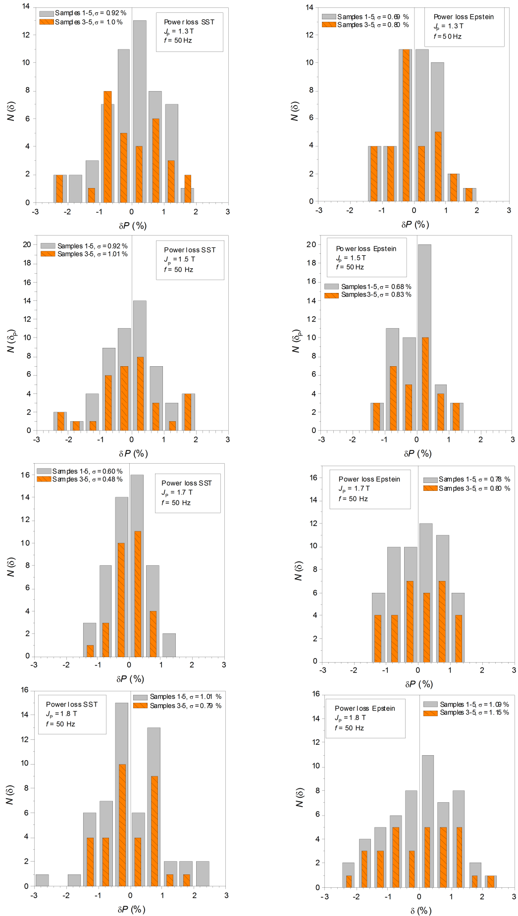
Fig. 6 – Dispersion of the laboratories best estimates of SST and Epstein power losses P_i at 50 Hz. The frequency N(\delta) of the relative differences \delta(P_i) is shown for the four investigated J_p levels. The response of the HGO samples (#3, #4, #5) is separately put in evidence.
