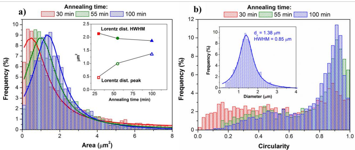
Figure 2. a) Islands area distribution formed at T_A = 870 °C and for different t_A fitted with the corresponding Lorentz curve (solid line); inset: evolution of peak and HWHM of Lorentz curve as a function of t_A . b) Islands circularity distribution formed at T_A = 870 °C and for different t_A ; inset: islands diameter distribution formed at T_A = 870 °C for t_A = 100 minutes with the corresponding Lorentz curve (solid line).
