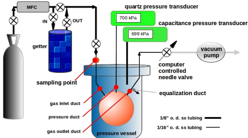
Figure 9. Scheme of the pressure and flow measurement control system.
