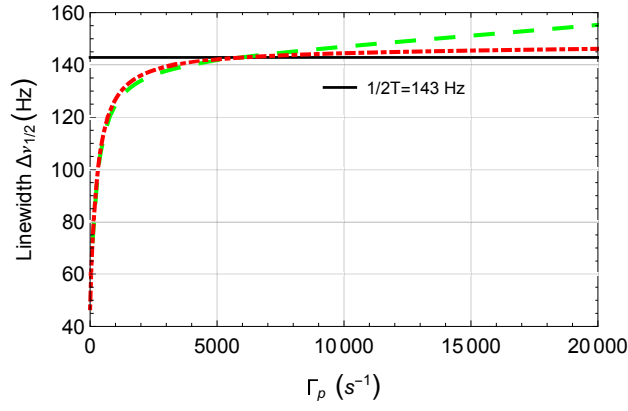
FIG. 3: (Color online) Calculated linewidth of the central Ramsey fringe versus \Gamma_p ; \gamma_2 = 300 \text{ s}^{-1} ; T = 3.5 \text{ ms} ; dashdot line: \tau_2 = 10 \text{ } \mu\text{s} ; dash line: \tau_2 = 100 \text{ } \mu\text{s} .
