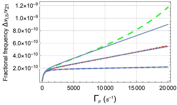
FIG. 4: (Color online) Calculated light-shift of the central Ramsey fringe versus \Gamma_p ; \gamma_2 = 300 \text{ s}^{-1} ; T = 3.5 \text{ ms} ; \Gamma^* = 2\pi \times 684 \text{ MHz} ; small dash line: \tau_2 = 5 \mu\text{s} ; dashdot line: \tau_2 = 50 \mu\text{s} ; large dash line: \tau_2 = 100 \mu\text{s} . For each curve, the approximated expression of the shift given by Eq. (19) has been superimposed to the numerically calculated behavior.
