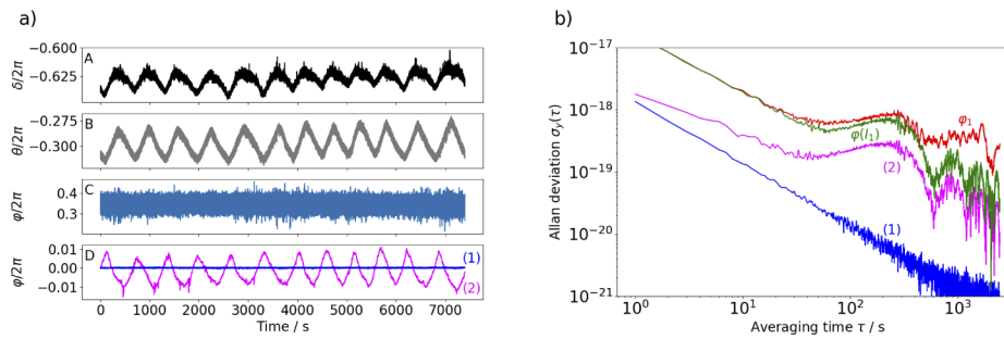
Fig. 3. Characterisation of the optical hybrid noise floor on a few-meters long optical link. (a) Panel A to C: the values of \delta , \theta and \phi as retrieved by the FPGA connected to the optical hybrid. Panel D: blue line (1), difference between the in-phase and quadrature component along the same axis; magenta line (2), difference between two in-phase components along x and y axes. (b) Corresponding frequency instabilities. Blue line (1) and magenta line (2), as in (a); green line ( \phi(I_1) ), phase detected by a single photodiode of the optical hybrid; red line ( \phi_1 ): out of loop phase between Slave Laser 1 and Master Laser.
