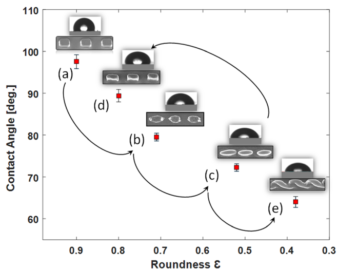
FIG. 2. Mean contact angle as a function of the micro-pillar roundness. Data points correspond to (a) as-fabricated sample; (b) first step of elongation (3 s irradiation); (c) second step of elongation (8 s irradiation); (d) recovery of the initial shape; and (e) irreversible elongation. In the insets, representative water droplet images and SEM images corresponding to each micro-pillar arrangement are shown.
