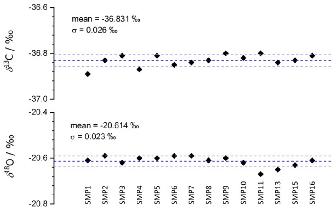
Figure 5: measurements of \delta^{13}\text{C} (top plot) and \delta^{18}\text{O} (bottom plot) on the same \text{CO}_2 source sampled via all 14 ports of the carousel. Each individual point represents the measurements via one port. The dashed and dotted lines represent the mean and standard deviation respectively.
