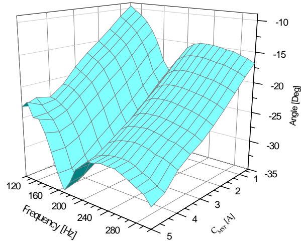
Figure 4. a) Function a_{\text{meas}} = \Gamma(C_{\text{MST}}, f) and b) function \beta = \beta(C_{\text{MST}}, f) , measured in the actual set-up.
