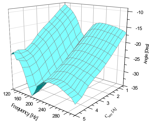
Figure 4. a) Function a_{meas} = \Gamma(C_{MST}, f) and b) function \beta = \beta(C_{MST}, f) , measured in the actual set-up.
