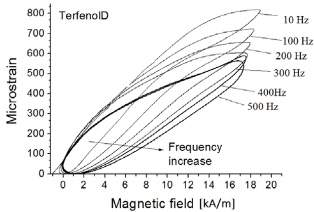
Figure 2. Dynamic magneto-mechanical characteristics of a Tb_{0.3}Dy_{0.7}Fe_{1.92} rod, based on the experimental identification of a CMP magnetostrictive model –Bottauscio et al. (2011). A constant magnetic bias of about 10 kA/m is provided through a DC current in a coil surrounding the material (preload: 8 MPa).
