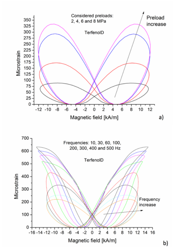
Figure 1. Dynamic magneto-mechanical characteristics of a \text{Tb}_{0.3}\text{Dy}_{0.7}\text{Fe}_{1.92} rod, based on the experimental identification of a CMP magnetostrictive model –Bottauscio et al. (2011). No magnetic bias is present. a) frequency: 300 Hz, b) preload: 8 MPa.
