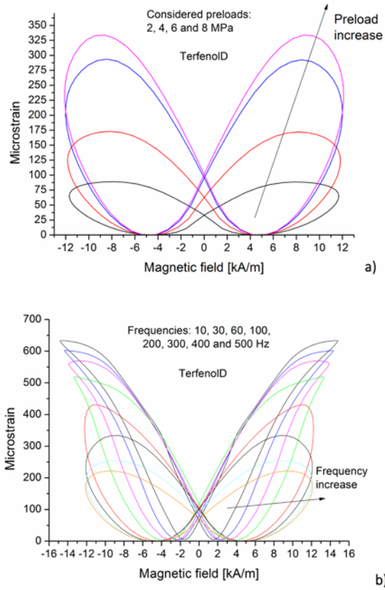
Figure 1. Dynamic magneto-mechanical characteristics of a Tb_{0.3}Dy_{0.7}Fe_{1.92} rod, based on the experimental identification of a CMP magnetostrictive model –Bottauscio et al. (2011). No magnetic bias is present. a) frequency: 300 Hz, b) preload: 8 MPa.
