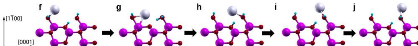
Figure. 5 Ball and stick representations of the diffusion mechanism of an Ag atom at the bare (a-e) and H 2 O covered (f-j) ZnO(110) surface in the [0001] direction (side view). Zinc, oxygen, hydrogen and silver atoms are represented respectively in magenta, red, cyan and gray. When moving on the H 2 O covered surface (f-j), the silver atom is always attached to a water molecule. This Ag-H 2 O bond has the double effect of flattening the PES and preventing the repulsive interaction between Ag and the surface Zn atoms.
