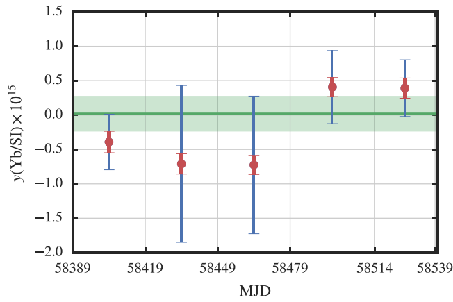
Figure 4. Fractional corrections y(f(Yb)/f(SI)) averaged every month of the campaign. Blue bars denote the total combined uncertainty, while red thick bars denote only the systematic contributions. The green shaded region denotes the weighted average for the campaign with its uncertainty.
