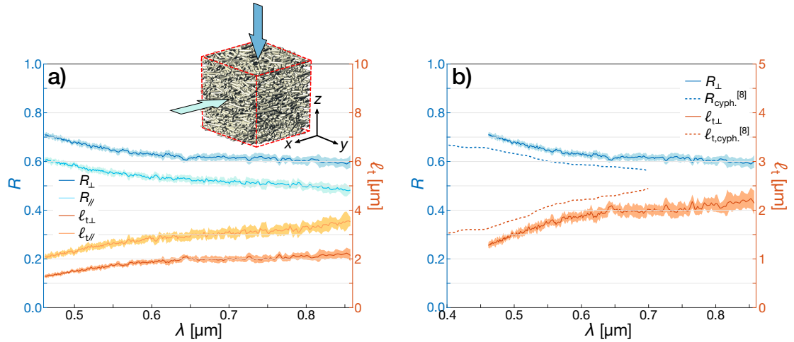
Figure 3: Calculated reflectance of an optimally scattering sample with \sigma_{\theta} = 0.2 rad and \varphi = 0.4 a) illuminated at perpendicular and parallel incidence, with corresponding l_t values retrieved from MC inversion and b) compared to the reflectance values obtained by FDTD calculations on the tomographic reconstruction of the Cyphochilus ultrastructure of the same size [8], showing a consistently higher reflectance in the visible range.
