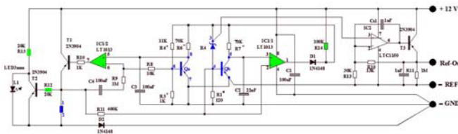
Fig. 1. – Electrical circuit of the Voltage Reference. The Heater is connected to the pins 1 and 2, while the Zener is connected to 3 and 4. Inside the chip there are also two transistors, the first to compensate the Zener temperature coefficient, the second act as a temperature sensor.
