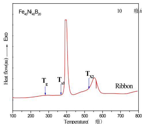
Figure 2. DSC curves of \text{Fe}_{40}\text{Ni}_{40}\text{B}_{20} amorphous ribbon
