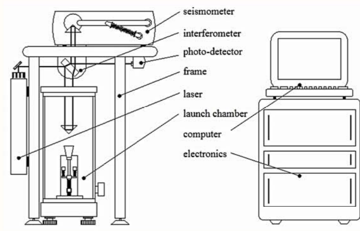
Schematic layout of the IMGC-02 absolute gravimeter
