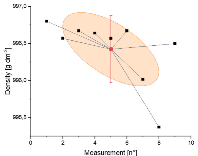
Fig. 4. MilliQ-H 2 O density results. Centroid point was evaluated, and the Y error bar corresponds to the SD of all measurements performed.
