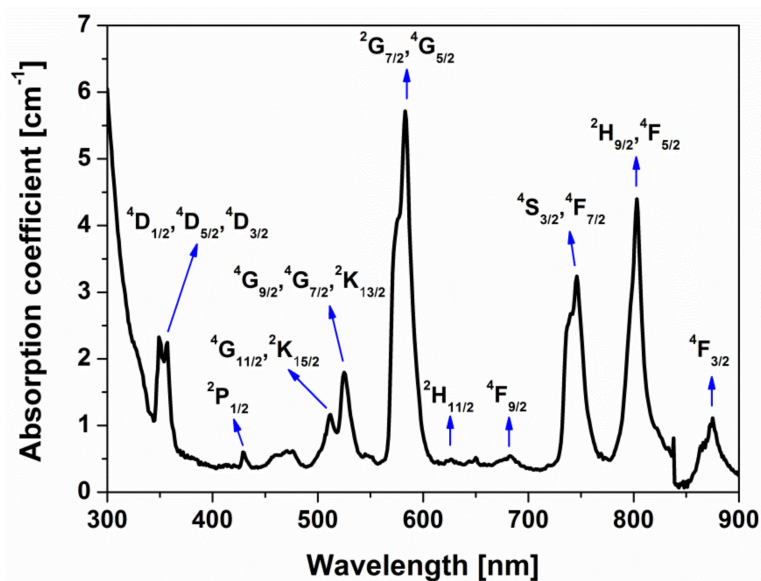
Figure 3. Absorption spectrum of the Nd-doped phosphate glass. The main \text{Nd}^{3+} levels are labeled, considering absorption from the ground state ^4I_{9/2} .
