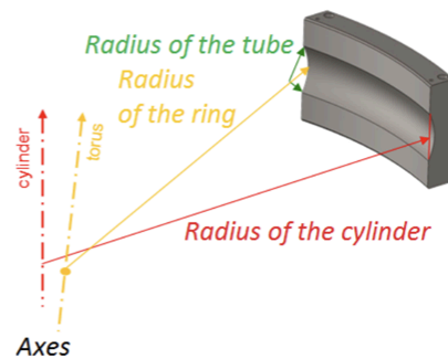
Figure 13: Large ring segment produced by MG Marposs, reported together with its form characteristics.
