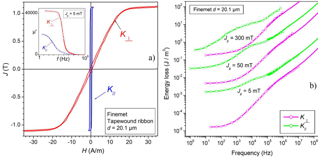
FIGURE 1. a) Quasi-static major hysteresis loops in a 20.1 \mu\text{m} thick tapewound nanocrystalline ribbon subjected to either longitudinal ( K_{//} ) or transverse ( K_{\perp} ) field annealing. The inset shows the frequency dependence of the associated initial permeabilities \mu'(f) (peak polarization J_p = 5 mT). b) Corresponding broadband energy loss behavior measured at three different J_p values. The dramatic decrease of the loss following the passage from the ( K_{//} ) to the ( K_{\perp} ) ribbons marks the transition from domain wall dominated ( K_{//} ) to rotation dominated ( K_{\perp} ) magnetization process.
