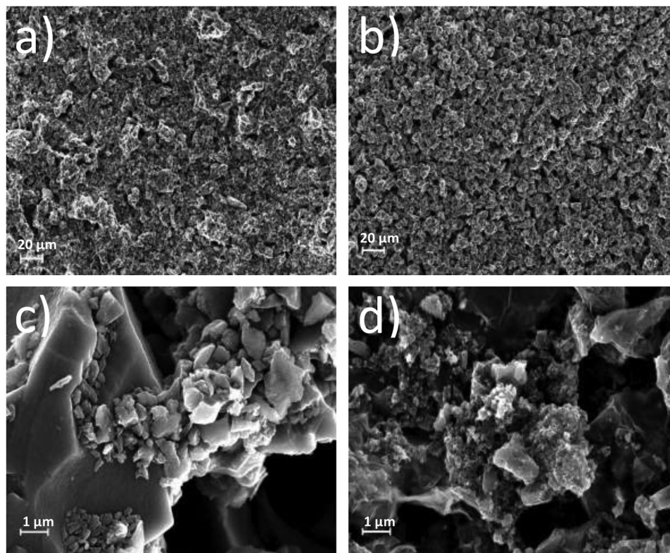
Figure 5. AC and PVDF network—magnification: a) 1000×, c) 25 000×. AC, GO, and PVDF networks—magnification: b) 1000× and d) 25 000×.
