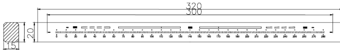
Main graduation : 280 mm length, 1 mm pitch, CD 4 \mu\text{m} , 1 mm line length
