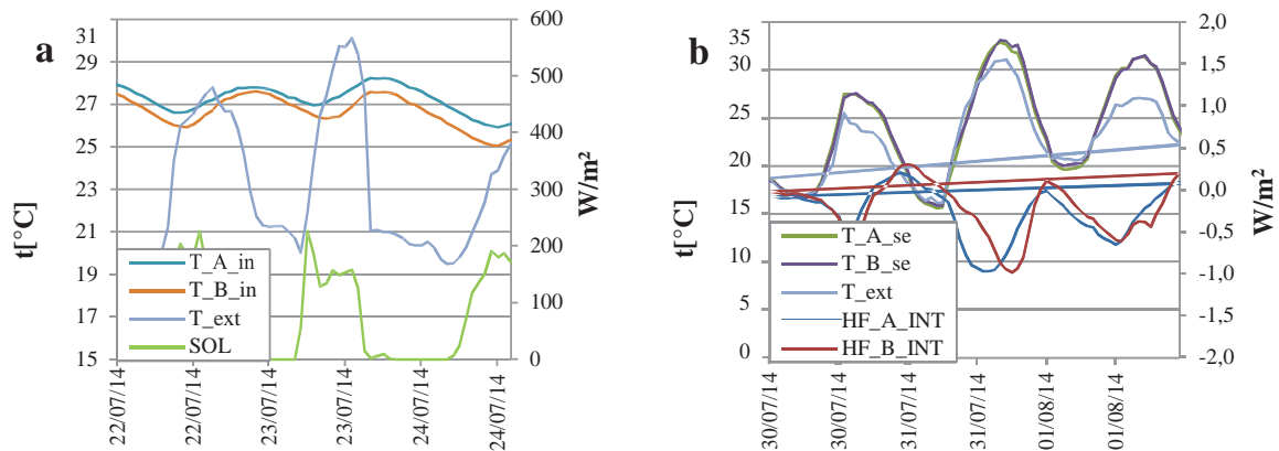
Figure 5. (a), (b) Summer measurement results. T_A_in is the air internal temperature in room A, T_B_in is the air internal temperature in room B, T_ext is the external temperature, SOL is the solar radiation irradiance, HF_A_INT is the heat flux measured on internal side in room A, HF_B_INT is the heat flux measured on internal side in room B, T_A_se is the external surface temperature of the room A, T_B_se is the external surface temperature of the room B.
