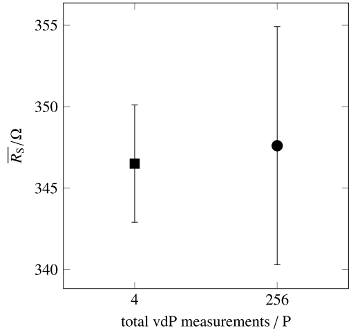
Fig. 7. Sheet resistance of sample S40 obtained with vdP measurements performed over 4 contacts ( P = 4 , square marker) and 16 contacts ( P = 256 , round marker). Error bars represent u(\overline{R_S}) .
