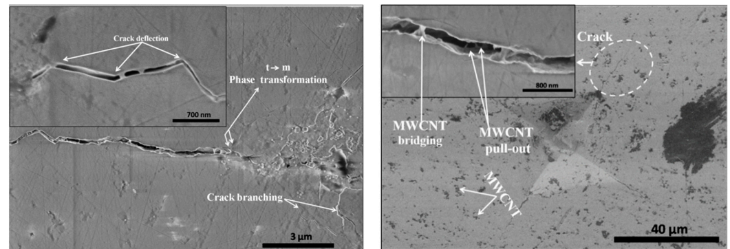
Figure 17. SEM micrographs showing toughening mechanisms in 8YSZ/1 wt% MWCNT composites. Adapted with permission from ref. [99], Copyright Elsevier 2019.
