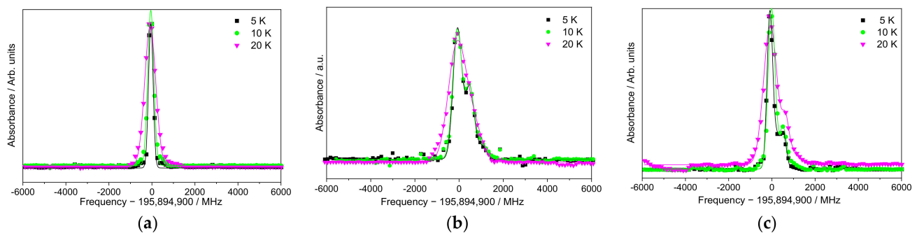
Figure 6. Er 3+ absorption spectra for transition ^4I_{15/2} \Gamma_{56}^{(1)} \rightarrow ^4I_{13/2} \Gamma_{78}^{(1)} at 5, 10, and 20 K for samples (a) ^{166}\text{Er}:^7\text{LiYF}_4 100 ppm; (b) Er:LiYF 4 100 ppm; (c) Er:LiYF 4 35 ppm.
