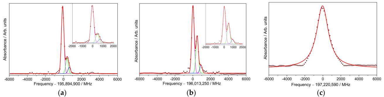
Figure 5. Er 3+ absorption spectra and their fitting of sample Er:LiYF 4 35 ppm for (a) ^4I_{15/2} \Gamma_{56}^{(1)} \rightarrow ^4I_{13/2} \Gamma_{78}^{(1)} ; (b) ^4I_{15/2} \Gamma_{56}^{(1)} \rightarrow ^4I_{13/2} \Gamma_{56}^{(1)} ; (c) ^4I_{15/2} \Gamma_{56}^{(1)} \rightarrow ^4I_{13/2} \Gamma_{78}^{(2)} . The red line is the total nonlinear fitting, the magenta, green, and blue lines are the individual peaks that contribute to the convolution.
