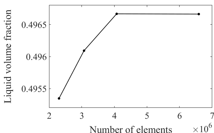
Figure A1. Liquid volume fraction for different grids at t = 10 s.
