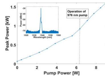
Fig. 4. Peak power of the optimal large core fiber (50 μm core diameter and 4 cm length). Inset: the spectrum.
