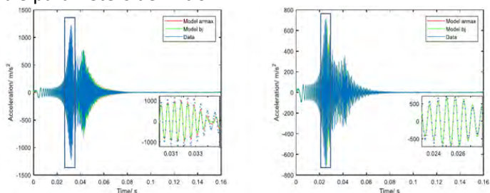
Figure 54 Experimental data and model fit of acceleration with 2kg (left) and 4 kg (right) top mass
